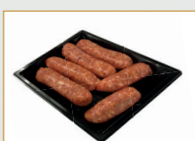
Chipolata worst
